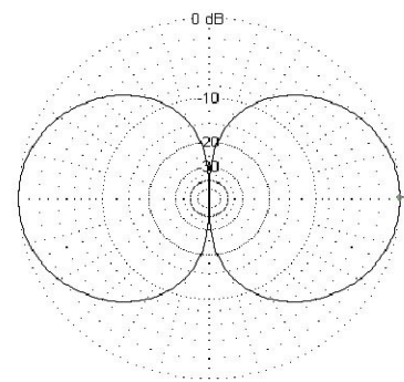
H PLANE 159 MHz
